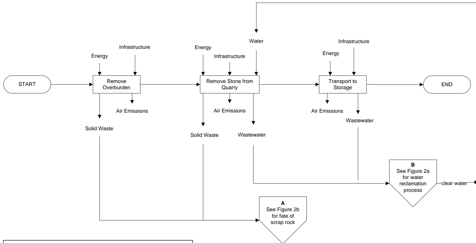
Figure 1. Quarry Operations Flow Diagram
